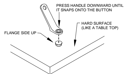
Figure 1: Assembly of Button into Holder
